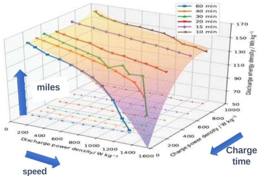
Figure 1. 3D Ragone plot of Samsung 30T cell
