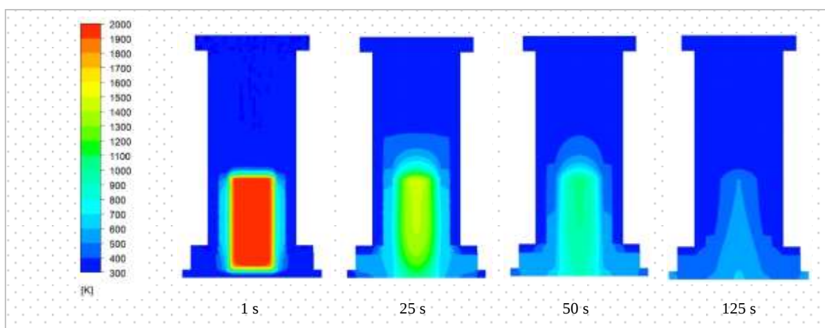
Figure 1. Temperature distribution in the central longitudinal section of the ESR mold.
