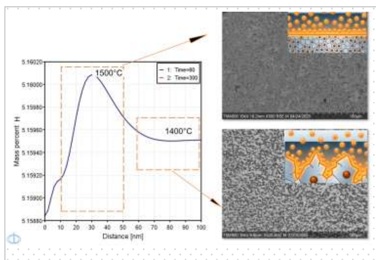
Figure 1 - Comparative analysis of hydrogen concentration profiles and hydrogen diffusion behavior in ODS steels consolidated at 1400 °C and 1500 °C.
